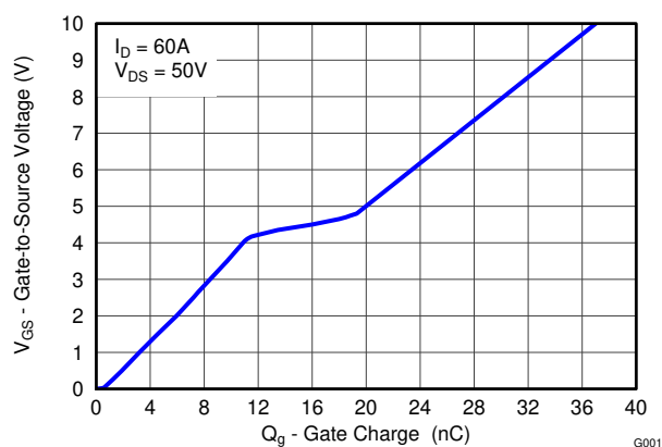
Gate Charge
