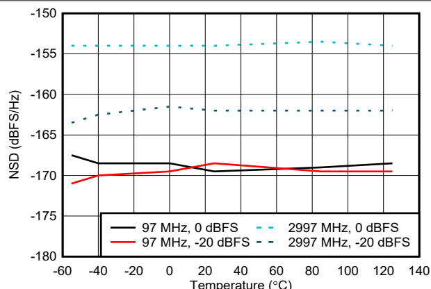
Figure 6-83. NSD vs Temperature
