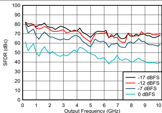
Figure 6-117. SFDR vs Frequency and Digital Amplitude in NRZ/RF Modes
