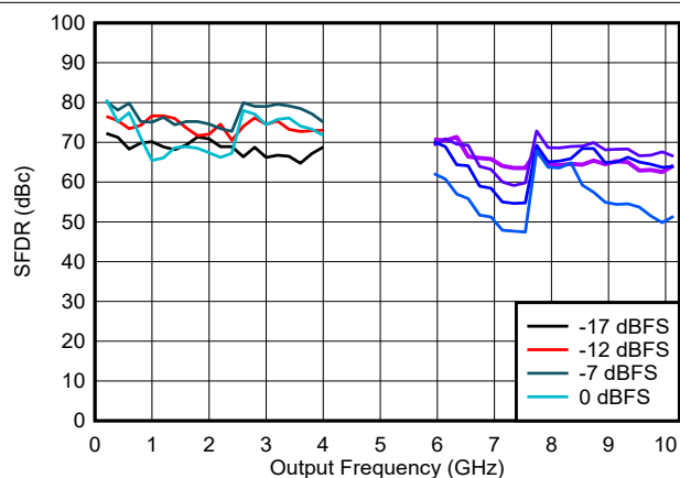
Figure 6-119. SFDR vs Frequency and Digital Amplitude in NRZ/RF Modes
