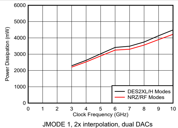
Figure 6-92. Power Dissipation vs Clock Frequency and DAC Mode
