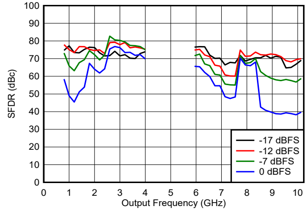
Figure 6-123. SFDR vs Frequency and Digital Amplitude in DES2X Modes
