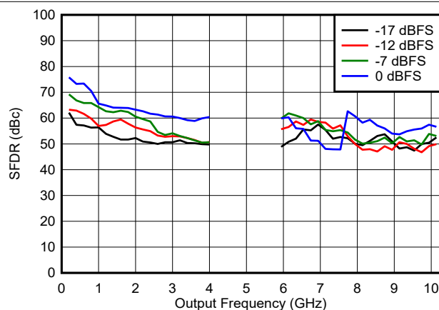
Figure 6-118. SFDR vs Frequency and Digital Amplitude in NRZ/RF Modes
