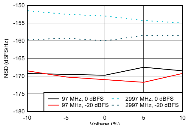
Figure 6-85. NSD vs Supply Voltage
