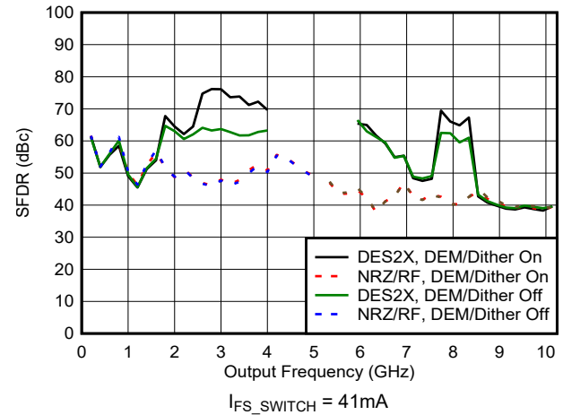
Figure 6-105. SFDR vs Frequency and Mode
