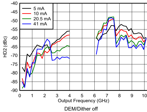
Figure 6-158. HD2 vs Frequency and Output Current in DES2X Modes
