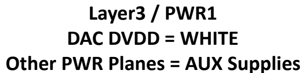
Figure 9-29. Power Plane Layout for Layer 3
