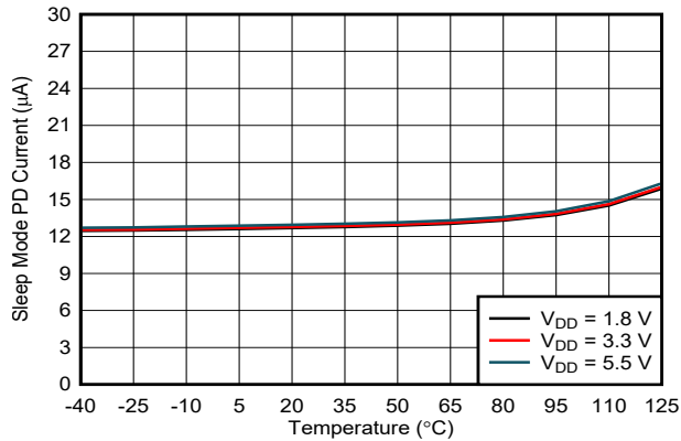
Figure 6-56. Power-Down Current vs Temperature
