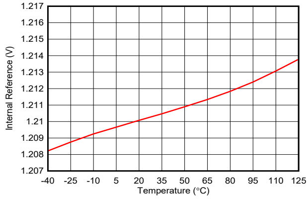
Figure 6-54. Internal Reference vs Temperature
