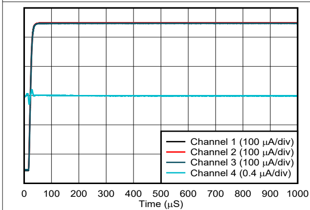
Channel 4 is resident, all other channels are interferers Figure 6-47. Current Output Channel-to-Channel Crosstalk
