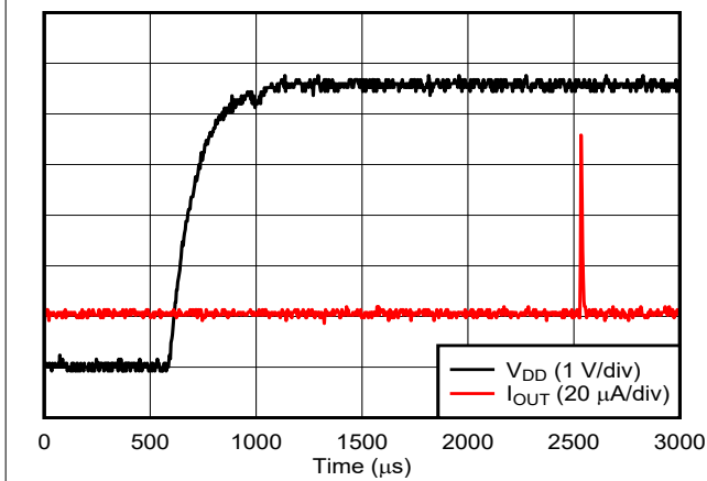
DAC at mid scale ( 0\ \mu\text{A} ) stored in EEPROM Figure 6-45. Current Output Power-On Glitch
