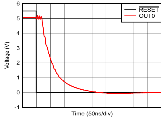
Figure 5-34. Power-On, Reset to Zero Scale
