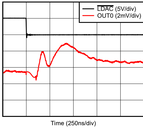
Figure 5-33. Glitch Impulse, Rising Edge
