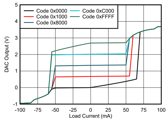
Figure 5-28. Source and Sink Capability
