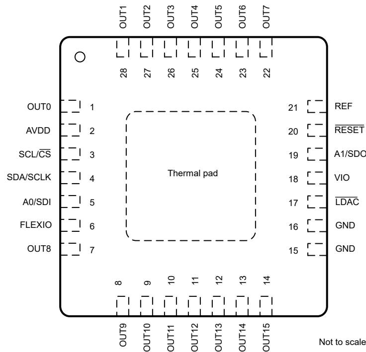
Figure 4-1. RUY Package, 28-Pin WQFN (Top View)
