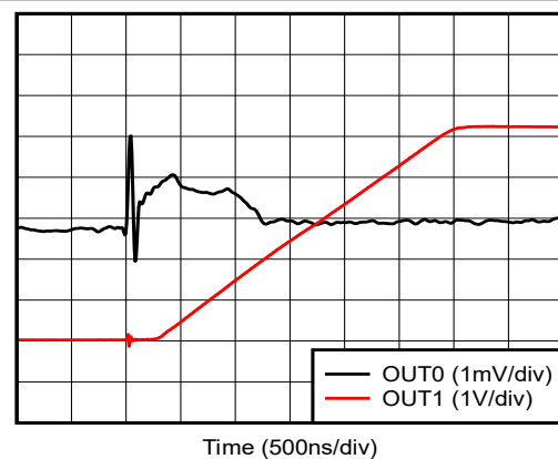
Figure 5-36. AV_{DD} Power Down Response
