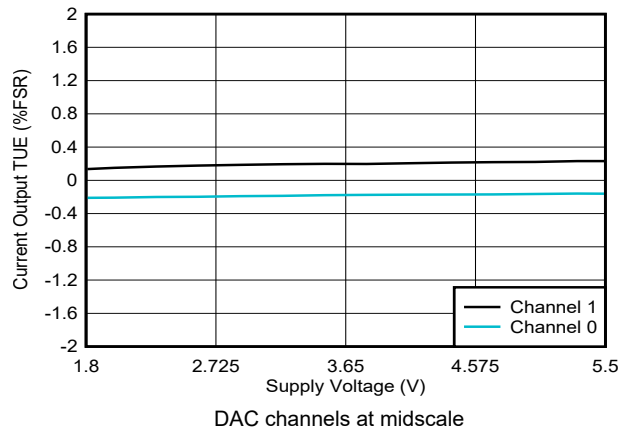
Figure 6-38. Current Output TUE vs Supply Voltage
