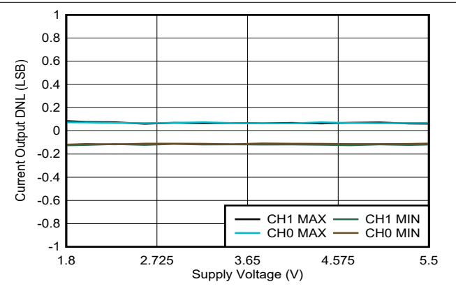
Figure 6-35. Current Output DNL vs Supply Voltage
