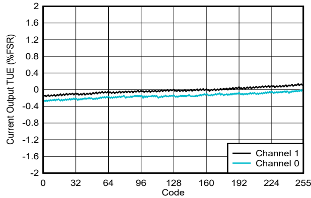
Figure 6-36. Current Output TUE vs Digital Input Code
