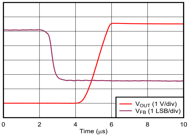
Comparator output in push-pull mode Figure 6-49. Comparator Response Time: Low-to-High Transition
