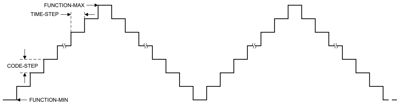
Figure 7-12. Triangle Waveform
