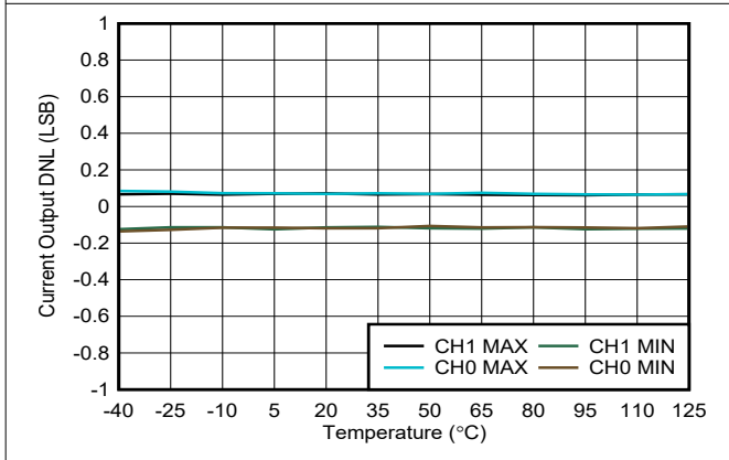
Figure 6-34. Current Output DNL vs Temperature
