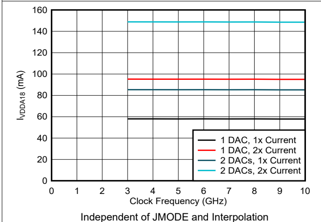
Figure 6-48. VDDA18 Current vs Clock Frequency and DAC Mode
