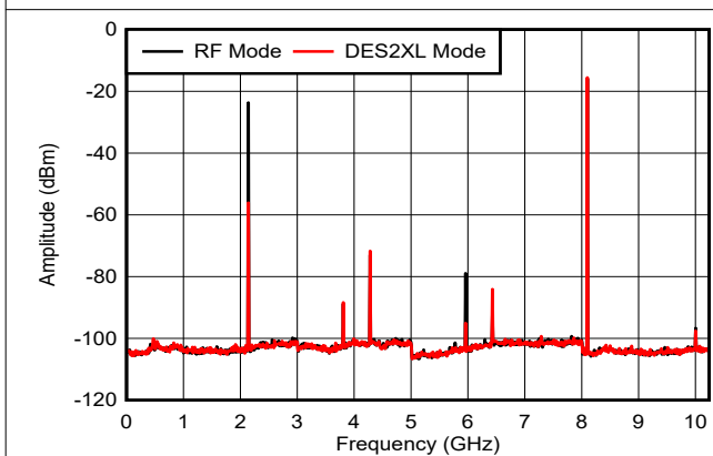
includes PCB, cable and balun loss Figure 6-24. f_{\text{OUT}} = 8097\text{MHz} , -6dBFS
