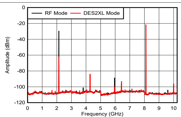
includes PCB, cable and balun loss Figure 6-25. f_{\text{OUT}} = 8097\text{MHz} , -12dBFS
