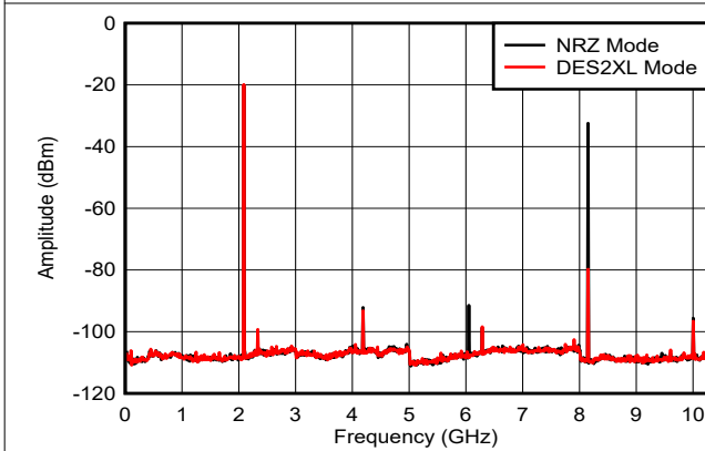
Figure 6-14. f_{\text{OUT}} = 2097\text{MHz} , 0dBFS
