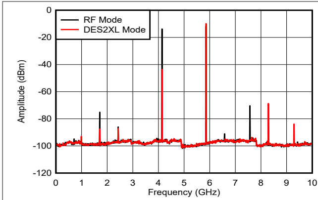
includes PCB, cable and balun loss Figure 6-20. f_{\text{OUT}} = 5997\text{MHz} , 0dBFS
