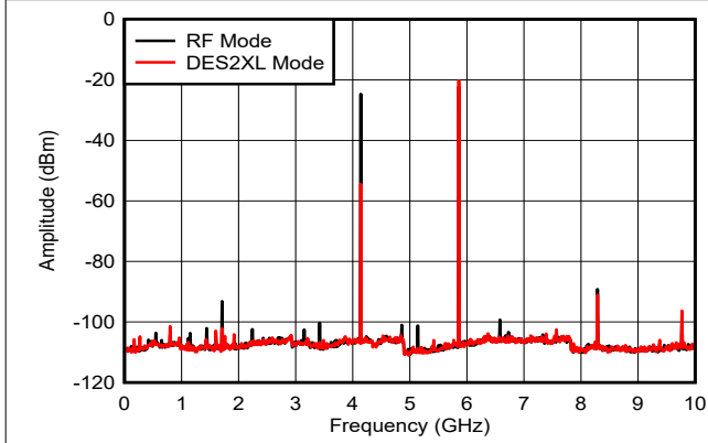
includes PCB, cable and balun loss Figure 6-22. f_{\text{OUT}} = 5997\text{MHz} , -12dBFS
