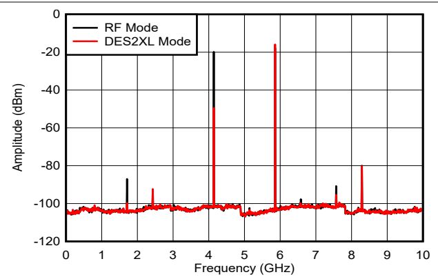
includes PCB, cable and balun loss Figure 6-21. f_{\text{OUT}} = 5997\text{MHz} , -6dBFS
