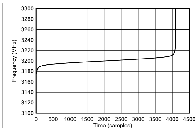
Figure 8-13. NLFM Frequency Ramp
