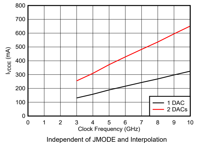
Figure 6-53. VDDE Current vs Clock Frequency
