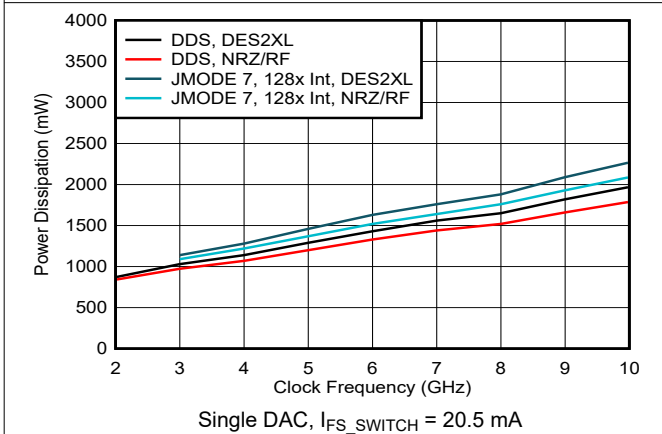
Figure 6-46. Power Dissipation vs Clock Frequency and Digital Mode
