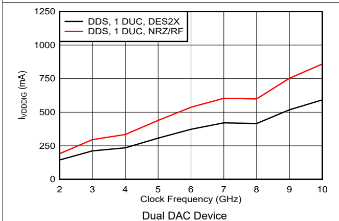
Figure 6-58. VDDDIG Current vs Clock Frequency and DAC Mode
