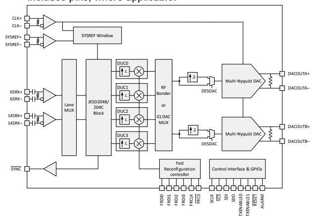
Block Diagram (Dual Channel Devices)
