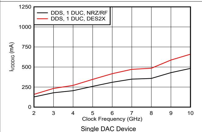
Figure 6-59. VDDDIG Current vs Clock Frequency and DAC Mode
