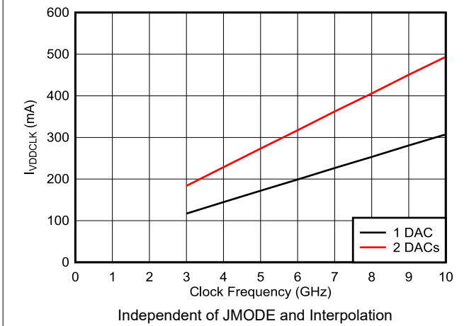
Figure 6-52. VDDCLK Current vs Clock Frequency
