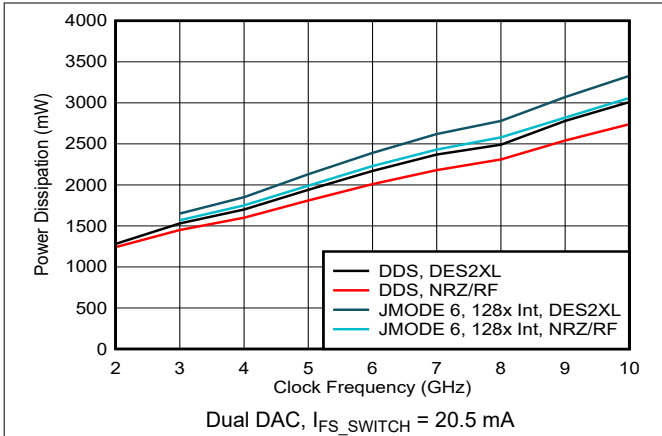
Figure 6-44. Power Dissipation vs Clock Frequency and Digital Mode
