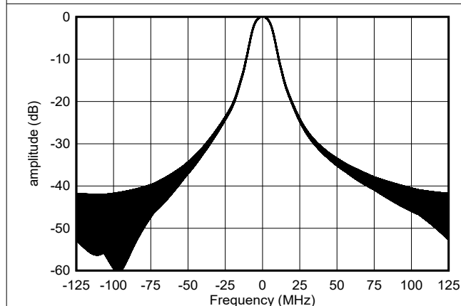
Figure 8-15. Digital Spectrum for NLFM Chirp
