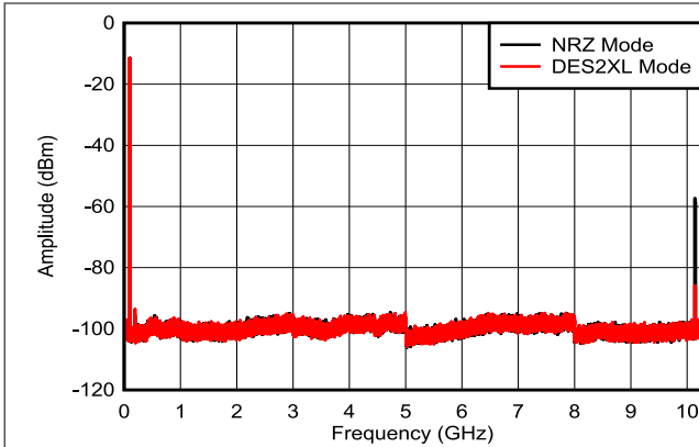
Figure 6-26. Dual Tone, f_{\text{OUT}} = 97\text{MHz} , 0dBFS
