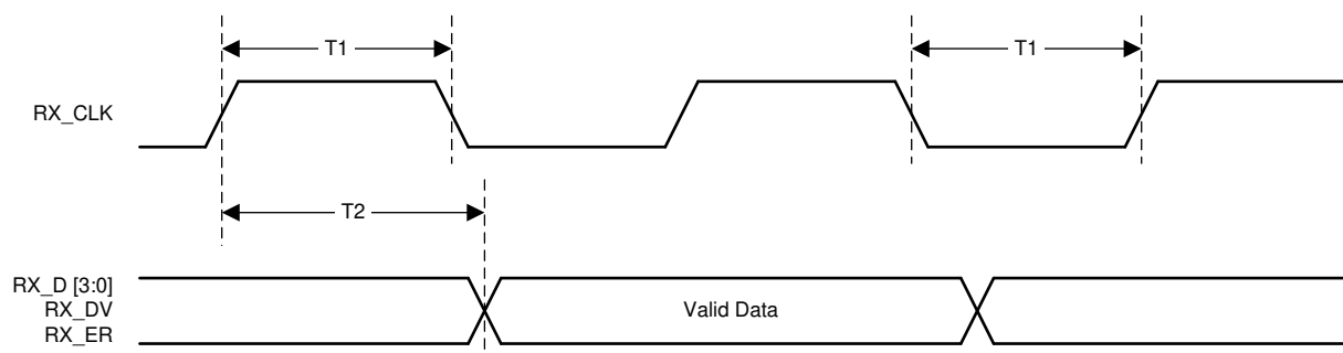
Figure 6-6. 100Mbps Receive Timing
