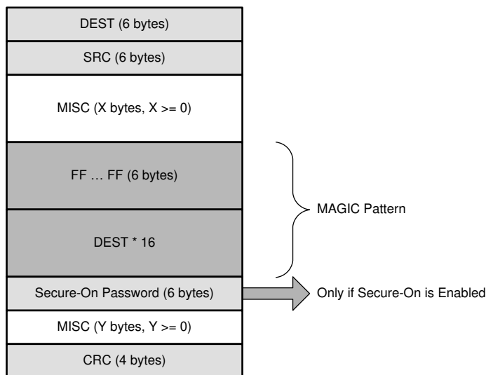
Figure 7-2. Magic Packet Structure
