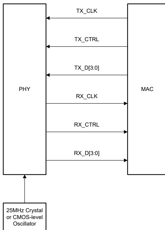
Figure 7-13. RGMII Connections
