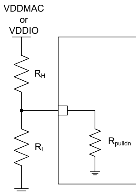
Figure 7-15. Strap Circuit
