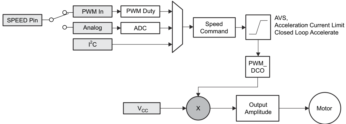
Figure 8-3. Multiplexing the Speed Command to the Output Amplitude Applied to the Motor
