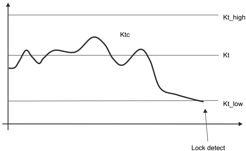
Figure 8-31. Abnormal-Kt Lock Detect
