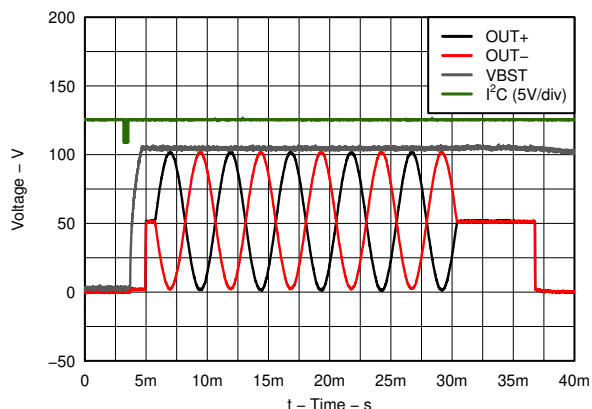
Figure 6-10. Typical Waveform
