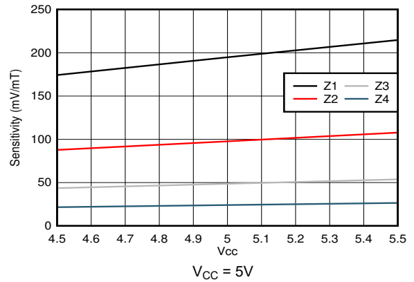
Figure 5-16. Sensitivity vs Supply Voltage
