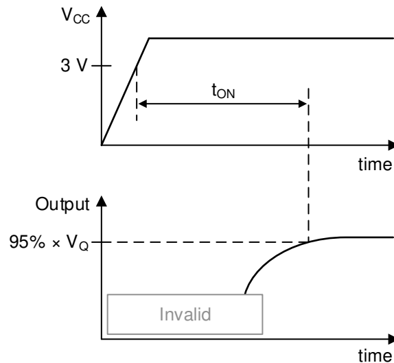
Figure 7-4. t_{ON} Definition
