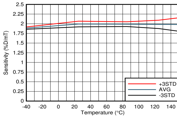
DRV5057Z1, V_{CC} = 5.0 V
