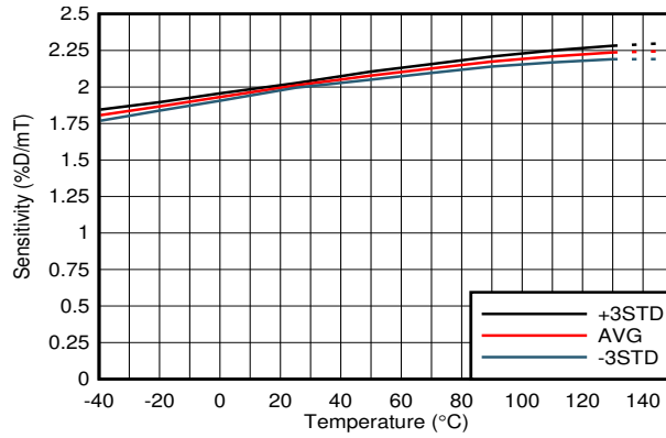
DRV5057A1, V_{CC} = 5.0 V
