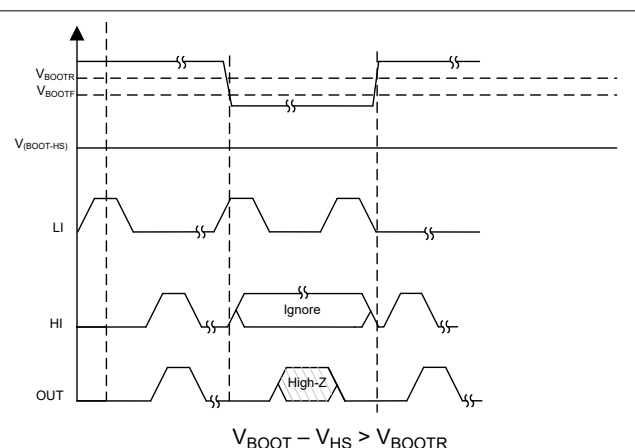
Figure 8-7. BOOT UVLO
