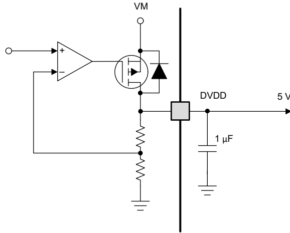
Figure 6-11. Linear Voltage Regulator Block Diagram
