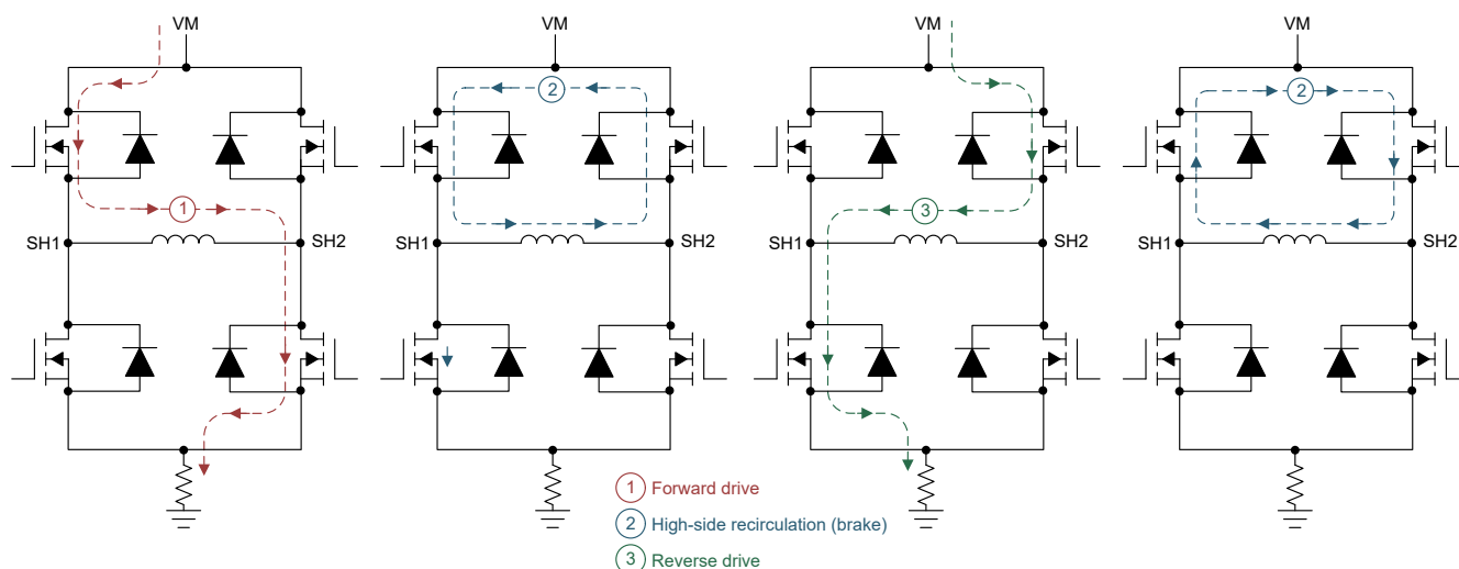
Figure 6-3. Current Paths
