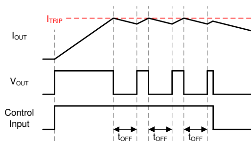
Figure 6-6. Current Regulation
