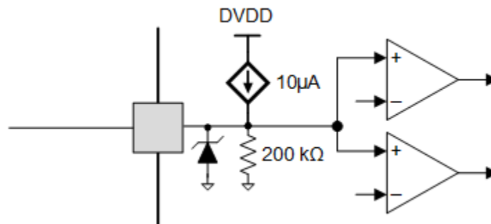
Figure 6-12. Tri-Level Input Pin Diagram
