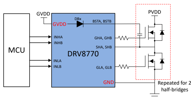
Simplified Schematic for DRV8770
