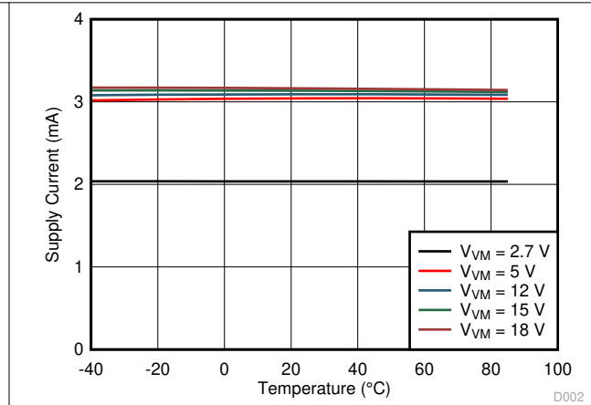
Figure 6-4. Operating Supply Current ( I_{VM} ) vs Ambient Temperature ( T_A )
