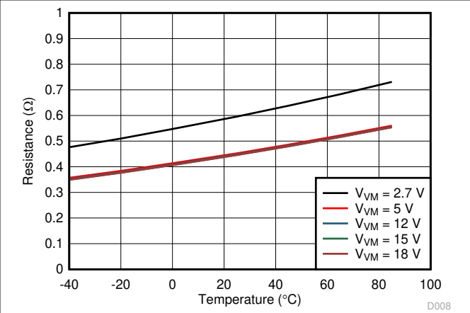
Figure 6-10. Low Side On-State Resistance ( R_{DS(ON)_LS} ) vs Ambient Temperature ( T_A )
