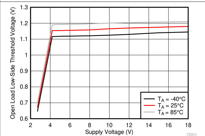
Figure 6-14. Open Load Low-Side Threshold Voltage ( V_{OL\_LS} ) vs Supply Voltage ( V_{VM} )
