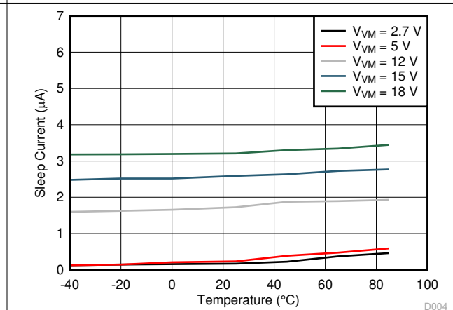
Figure 6-6. Sleep Mode Supply Current ( I_{VM0} ) vs Ambient Temperature ( T_A )
