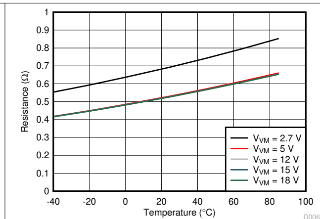
Figure 6-8. High Side On-State Resistance ( R_{DS(ON)_HS} ) vs Ambient Temperature ( T_A )
