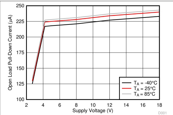
Figure 6-12. Open Load Pull-Down Current ( I_{OL\_PD} ) vs Supply Voltage ( V_{VM} )
