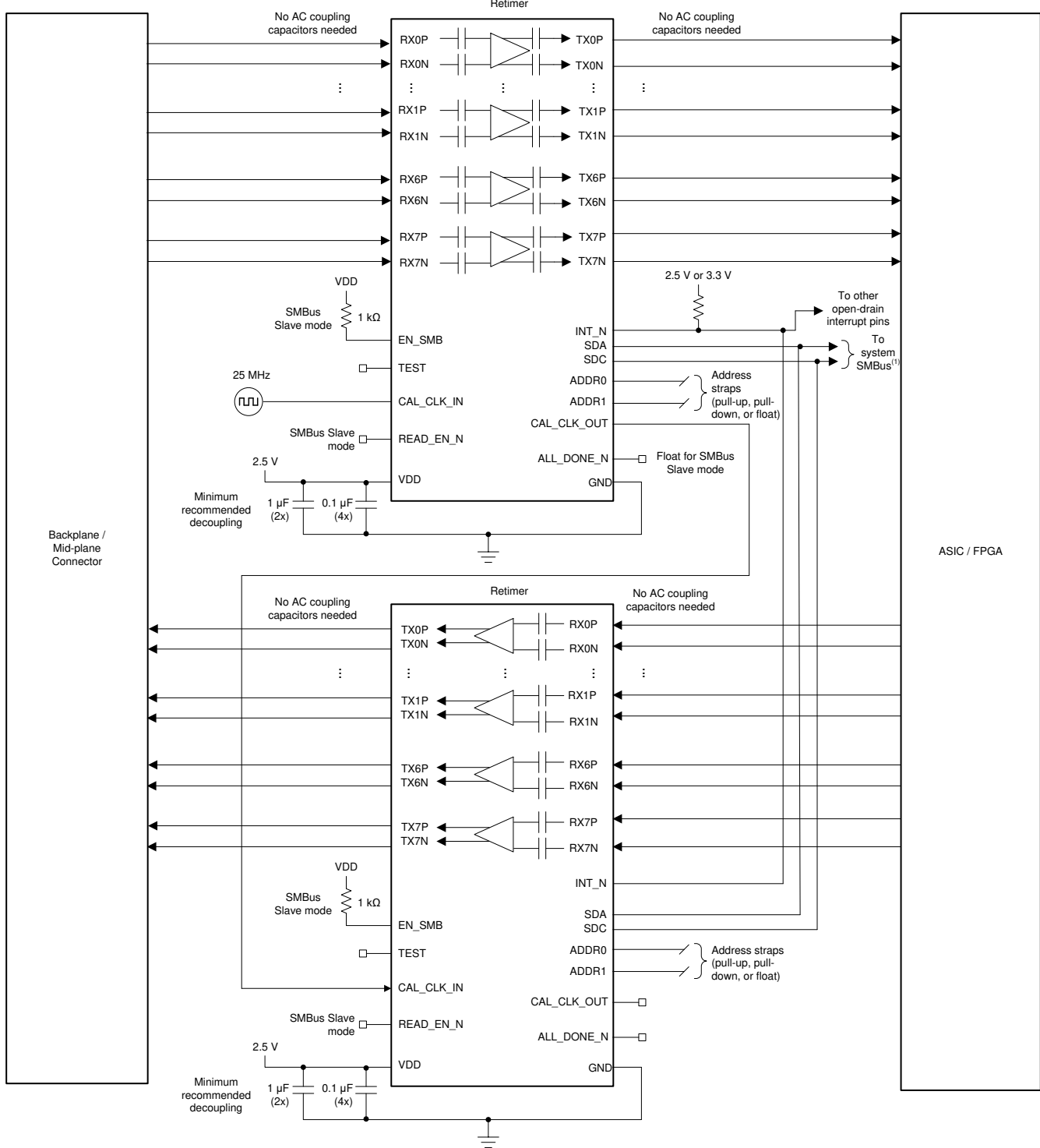
Figure 7-3. Backplane and Mid-Plane Application Schematic
