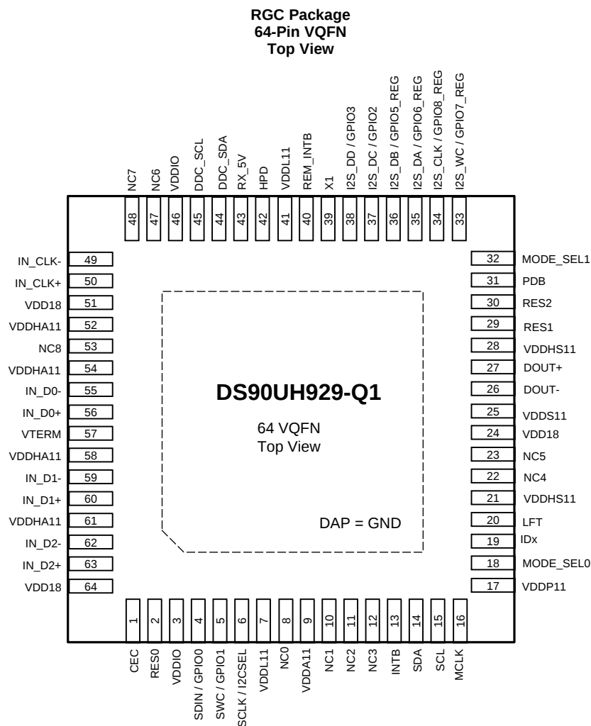
Pin Functions
