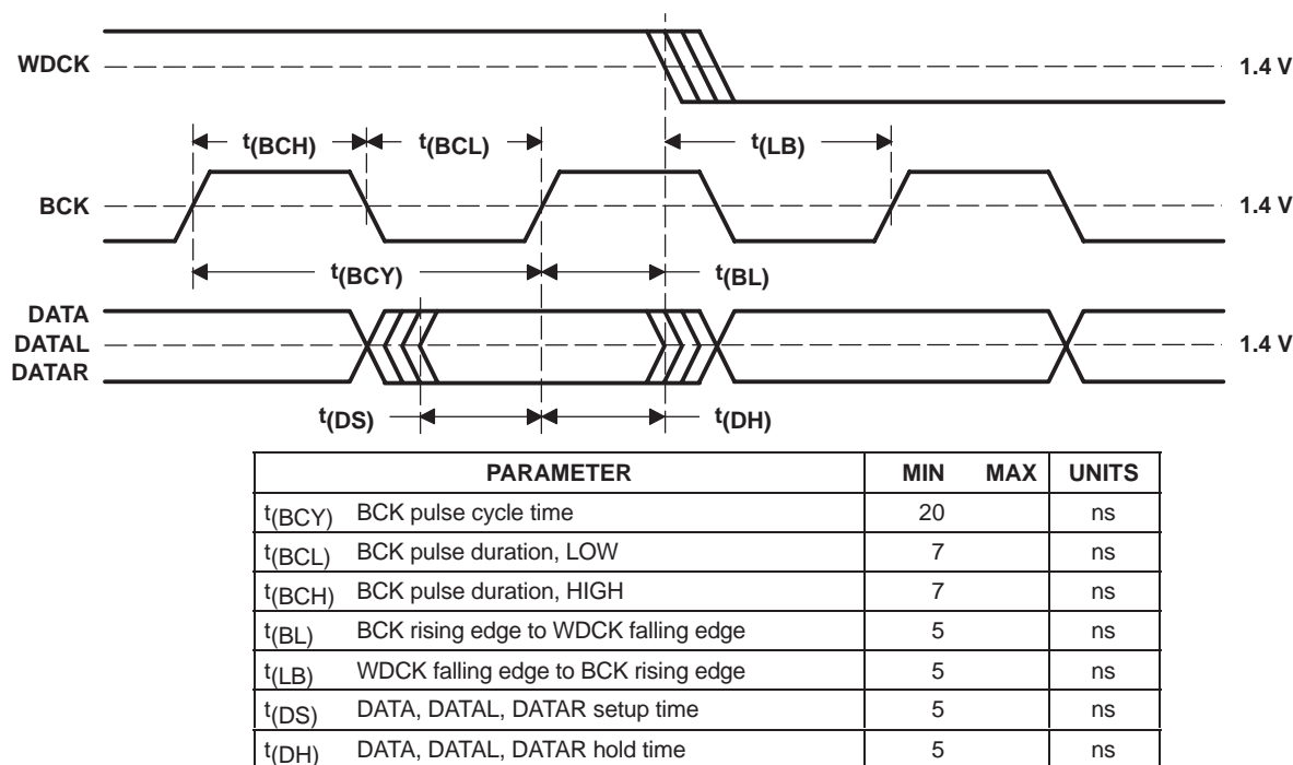
Figure 37. Audio Interface Timing for External Digital Filter (Internal DF Bypass Mode) Application
