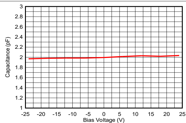
Figure 5-6. Bias Voltage vs Capacitance
