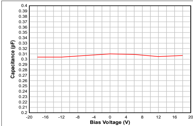
Figure 5-1. Bias Voltage vs. Capacitance
