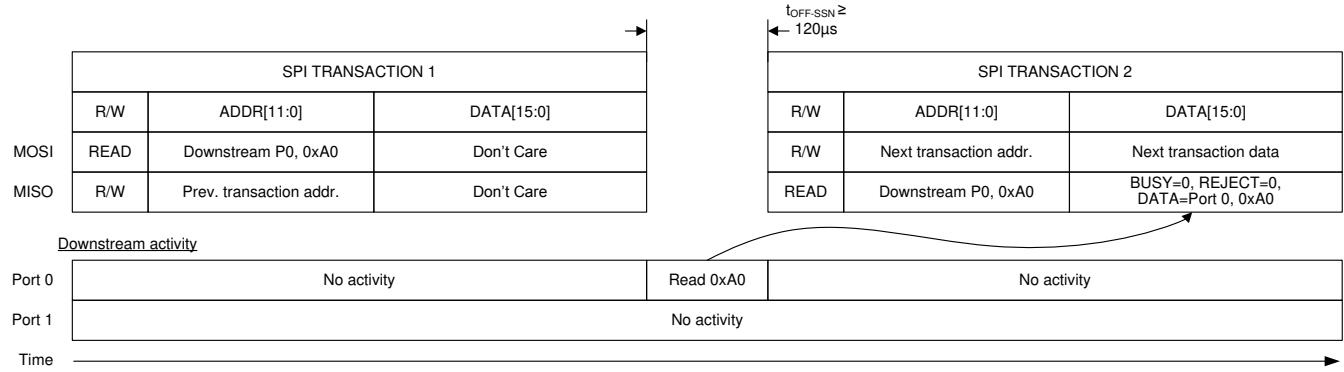
Figure 7-10. SPI Read Consisting of Two Separate SPI Transactions
