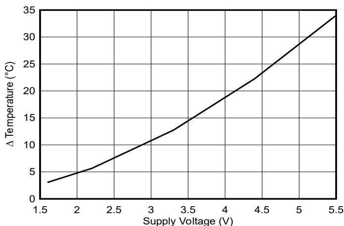
Figure 7-13. Heater Induced Temperature Increase vs Supply Voltage on a Rigid 1.575mm FR4 PCB
