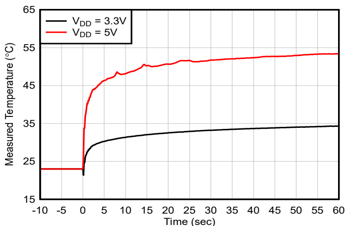
Figure 7-14. Heater Induced Temperature Increase on a Rigid PCB (1.575mm FR4)
