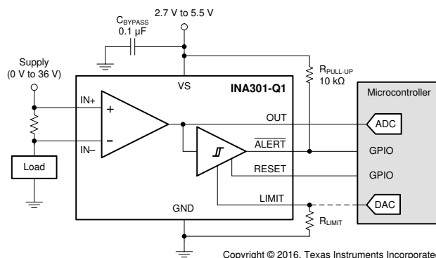
Typical Application
