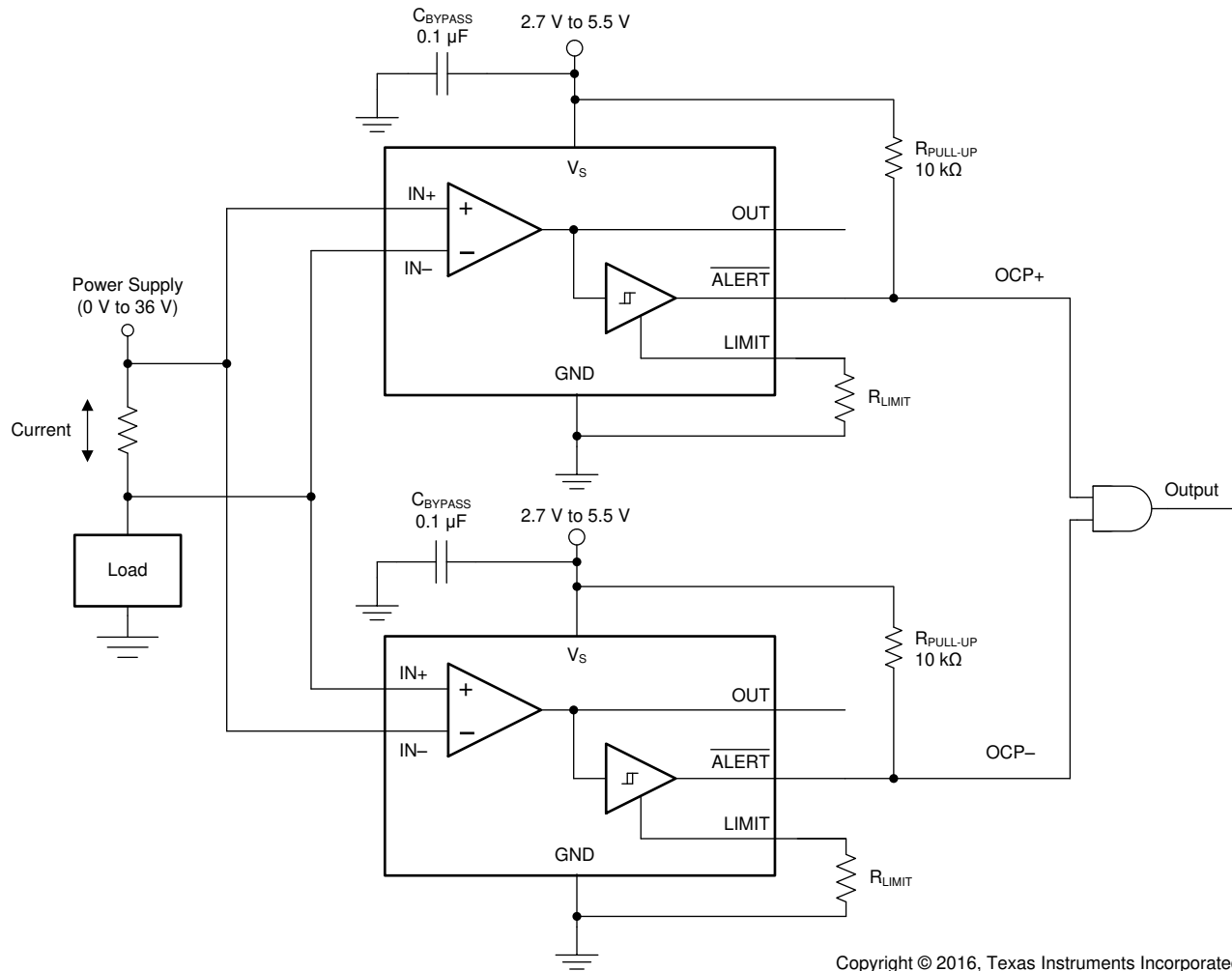
Figure 8-4. Bidirectional Application
