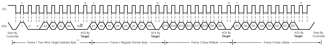
Figure 6-3. Timing Diagram for Write Word Format
