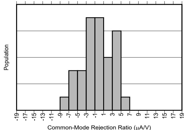
Figure 5-5. INA750A Common-Mode Rejection Production Distribution
