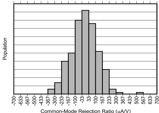
Figure 5-6. INA750B Common-Mode Rejection Production Distribution
