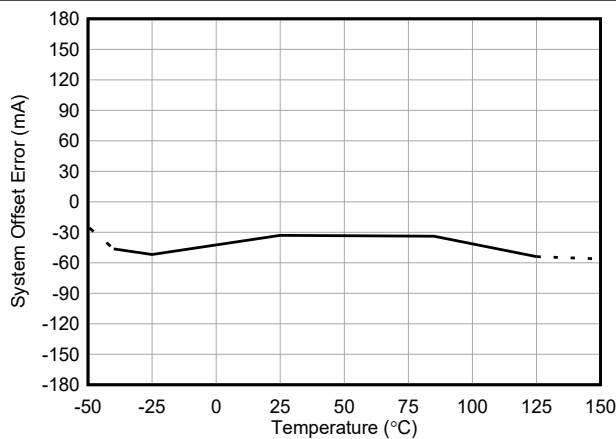
Figure 5-4. INA750B Input Offset Current vs Temperature
