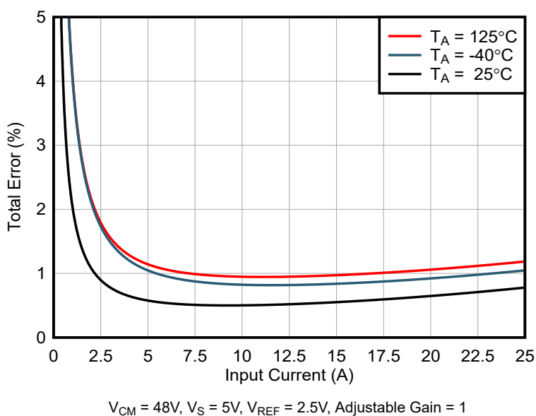
Figure 7-1. INA750A Total Error vs Input Current
