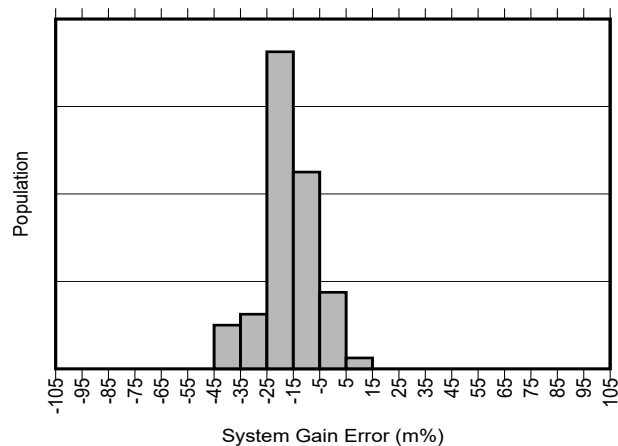
Figure 5-11. INA750A Gain Error Production Distribution
