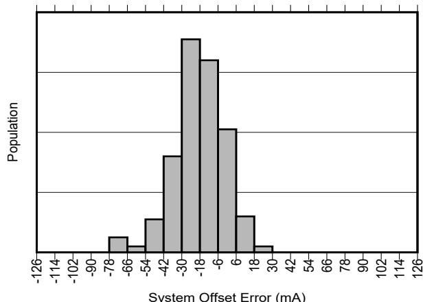
Figure 5-2. INA750B Input Offset Current Production Distribution
