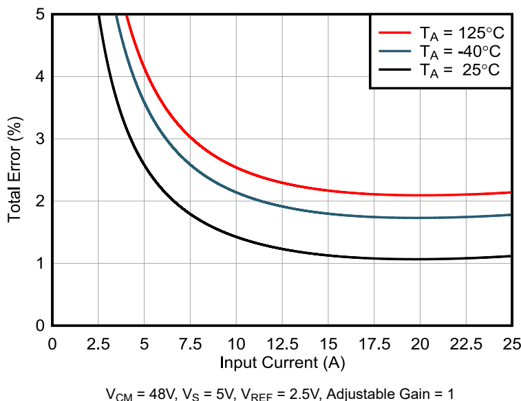
Figure 7-2. INA750B Total Error vs Input Current
