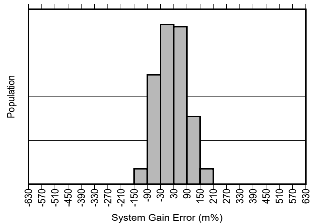
Figure 5-12. INA750B Gain Error Production Distribution
