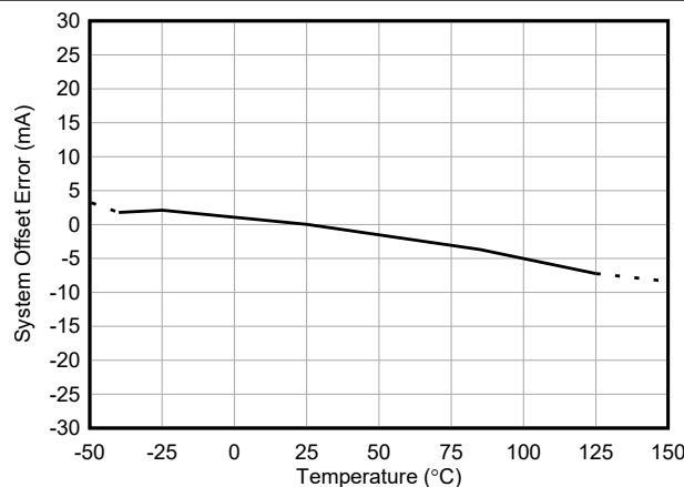
Figure 5-3. INA750A Input Offset Current vs Temperature
