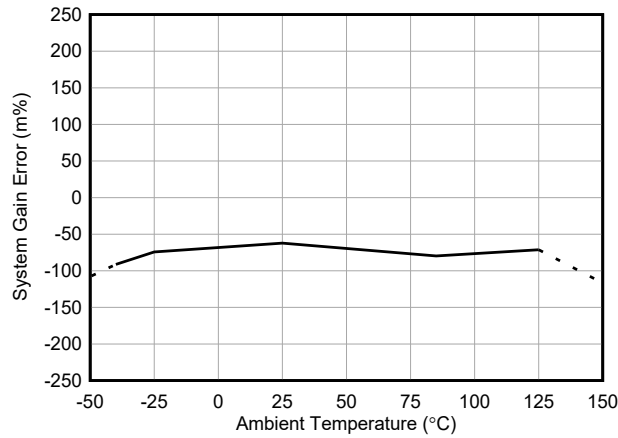
Figure 5-13. INA750A Gain Error vs Temperature
