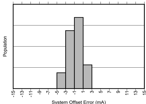
Figure 5-1. INA750A Input Offset Current Production Distribution
