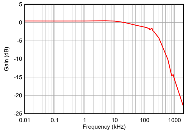
Figure 9-5. Bandwidth at R_L = 4.7\text{k}\Omega
