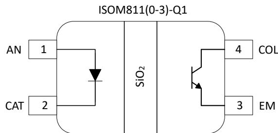
Figure 5-1. ISOM811[0-3]-Q1 4-Pin SOIC (Top View)
