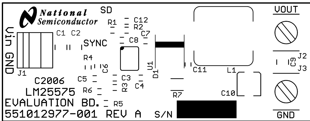
Figure 7-13. Silkscreen
