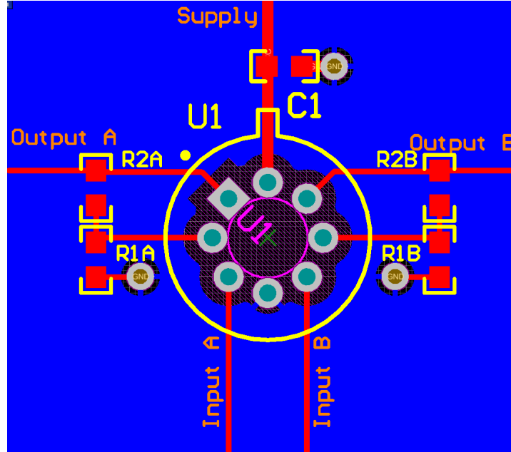
Figure 10-1. Layout Example
