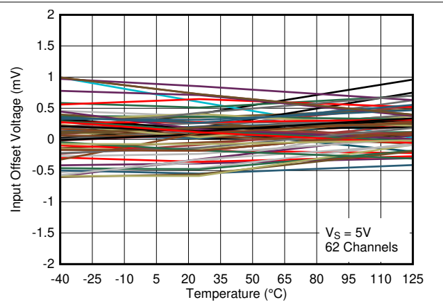
Figure 2-8. Input Offset Voltage vs. Temperature at 5V
