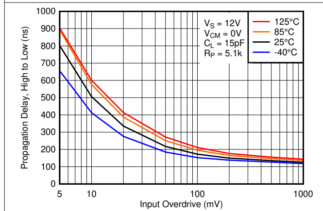
Figure 2-27. High to Low Propagation Delay vs. Input Overdrive Voltage, 12V
