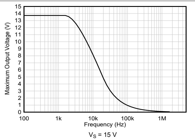
Figure 5-32. Maximum Output Voltage vs Frequency V_S = 15\text{ V}
