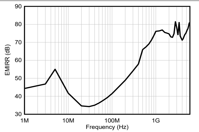
Figure 5-34. EMIRR (Electromagnetic Interference Rejection Ratio) vs Frequency
