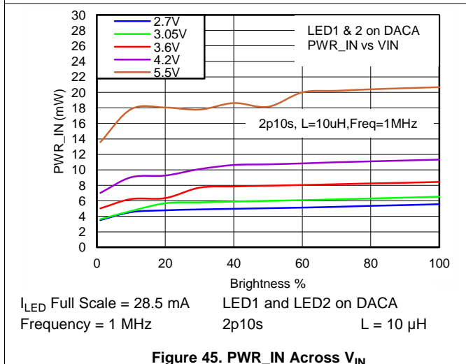
Figure 45. PWR_{IN} Across V_{IN}
