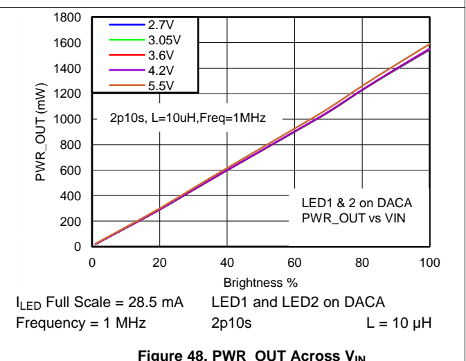
Figure 48. PWR_{OUT} Across V_{IN}
