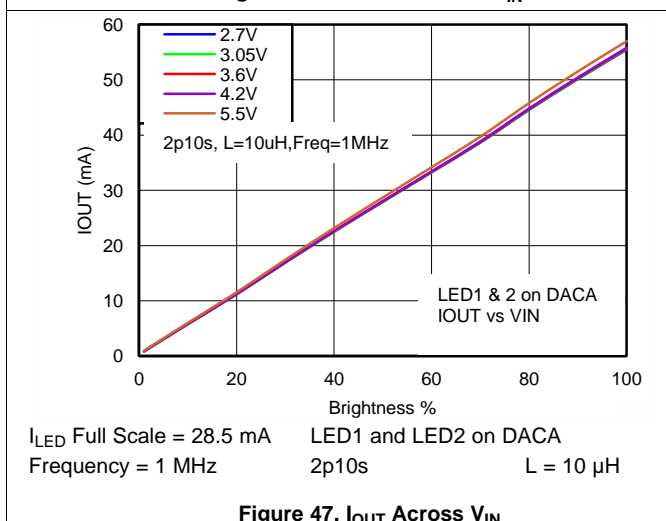
Figure 47. I_{OUT} Across V_{IN}
