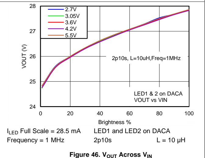
Figure 46. V_{OUT} Across V_{IN}
