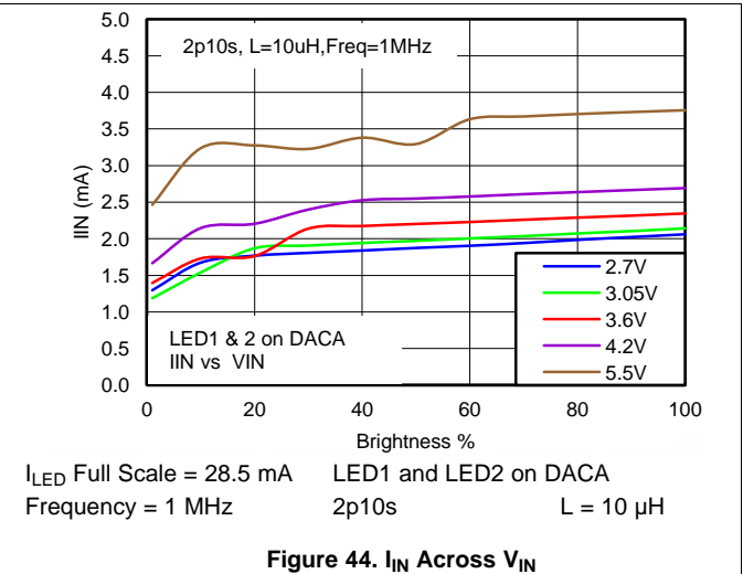
Figure 44. I_{IN} Across V_{IN}
