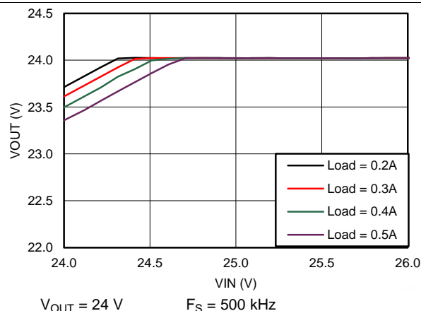
Figure 80. Dropout Curve
