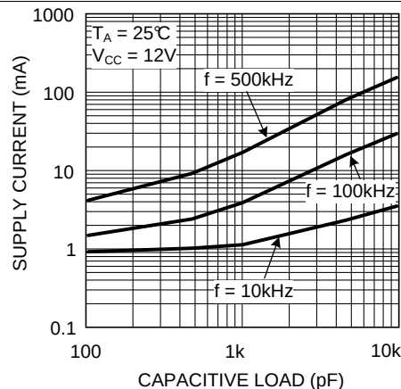
Figure 15. Operating Current vs Load Capacitance
