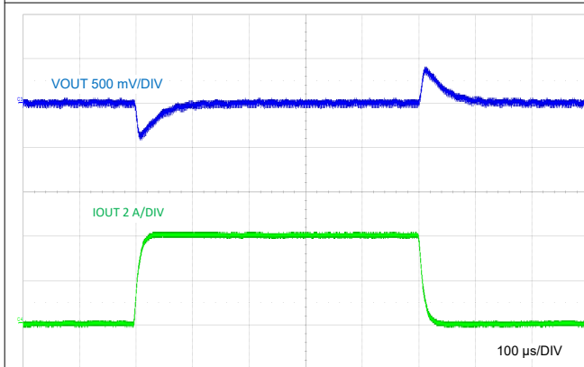
Figure 9-27. Load Transient, 0 A to 4 A
