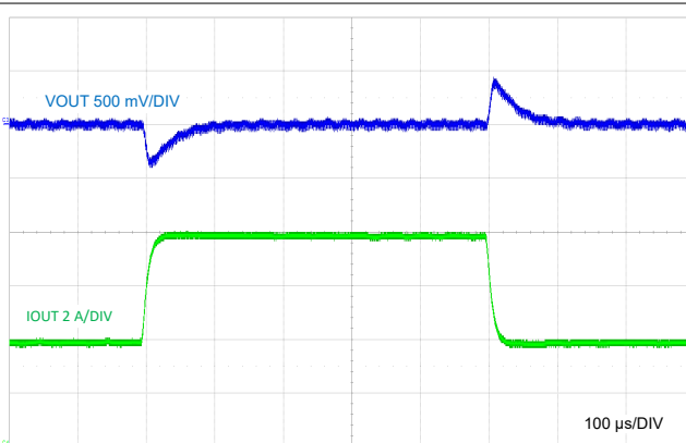
Figure 9-28. Load Transient, 4 A to 8 A
