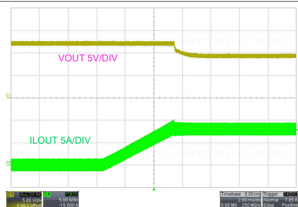
Figure 9-13. CV to CC Mode Transition, V_{\text{SUPPLY}} = 48\text{V} , V_{\text{LOAD}} = 12\text{V} to 9V
