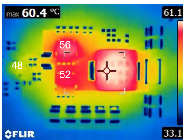
Figure 9-14. V_{\text{SUPPLY}} = 48\text{V} , I_{\text{LOAD}} = 8\text{A} , T_{\text{A}} = 25^{\circ}\text{C} , No Airflow
