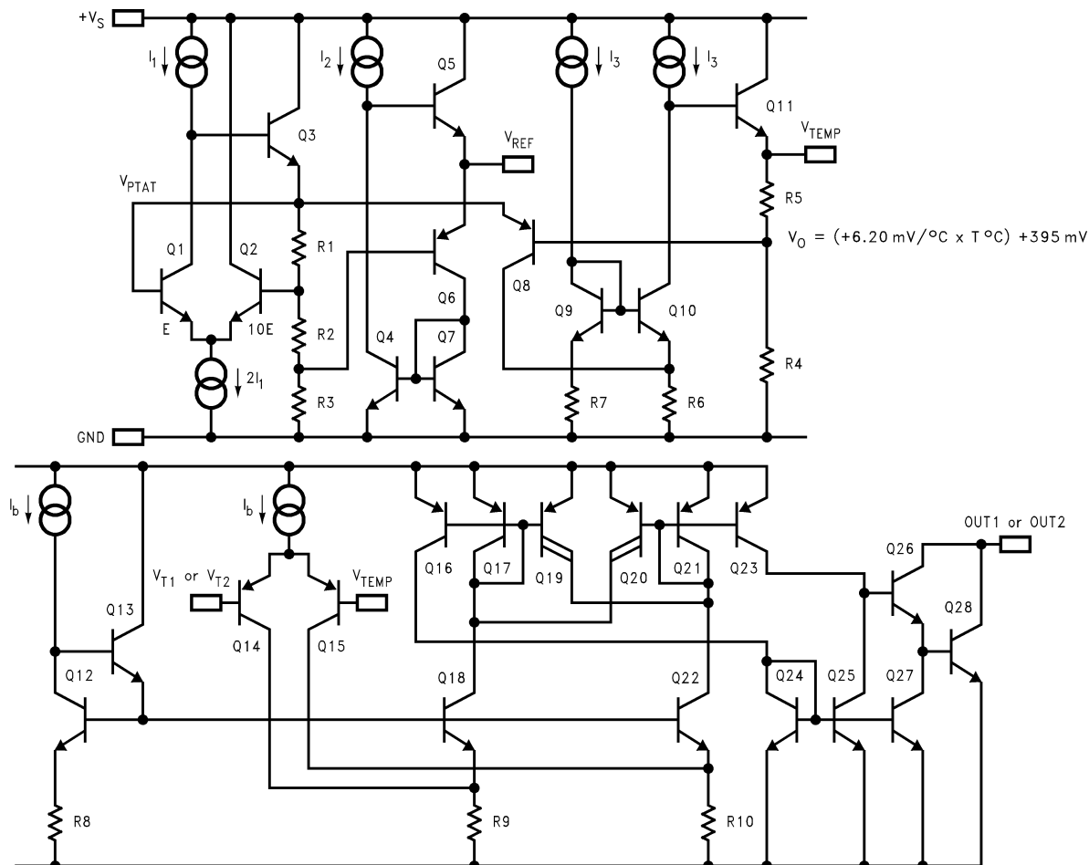
Figure 15. Simplified Schematic
