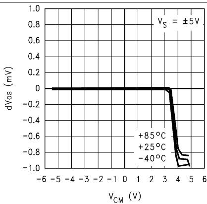
Figure 3. dV_{OS} vs. V_{CM}
