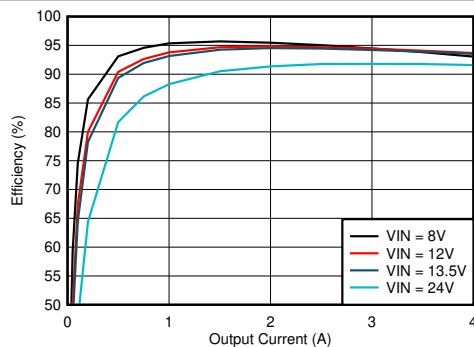
Figure 9-5. LM61440 Efficiency
