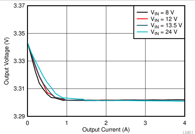
Figure 9-10. LM61440 Load and Line Regulation
