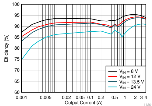
Figure 9-6. LM61440 Efficiency
