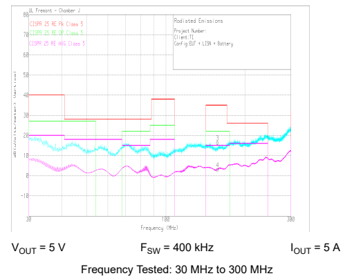
Figure 9-58. Radiated EMI Bicon Horizontal versus CISPR25 Limits
