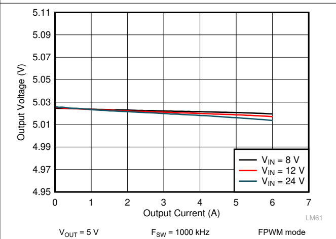
Figure 9-26. LM61460 Load and Line Regulation
