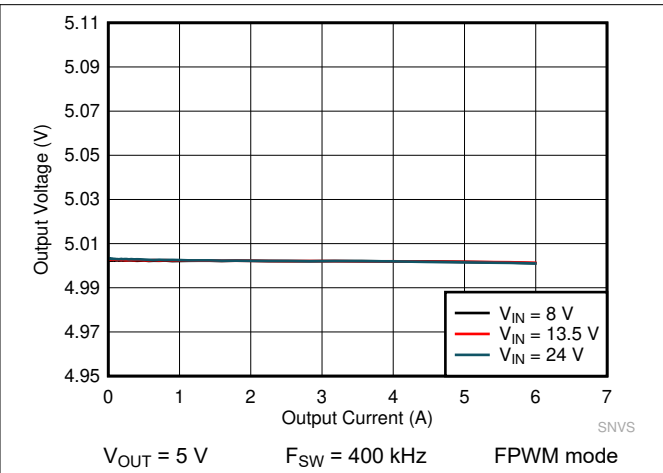
Figure 9-24. LM61460 Load and Line Regulation
