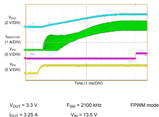
Figure 10-19. LM62440-Q1 Start-up with 3.25-A
