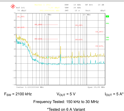
Figure 10-34. Conducted EMI versus CISPR25 Limits (Yellow: Peak Signal, Blue: Average Signal), LM61460EVM
