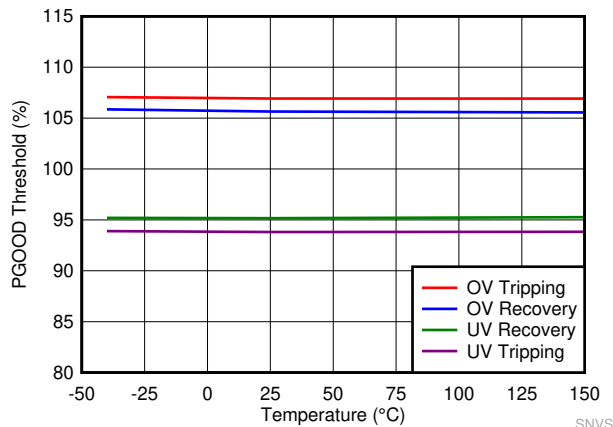
Figure 8-8. PGOOD Thresholds
