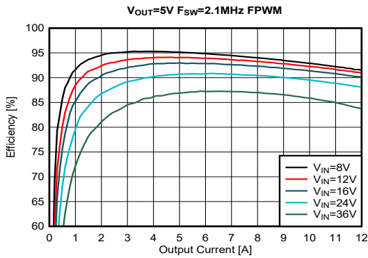
Figure 8-15. Efficiency
