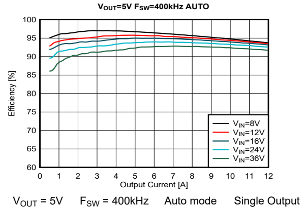
Figure 8-10. Efficiency
