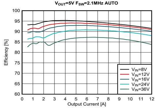
Figure 8-16. Efficiency
