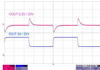
Figure 8-54. Load Transient
