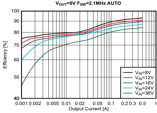
Figure 8-15. Efficiency
