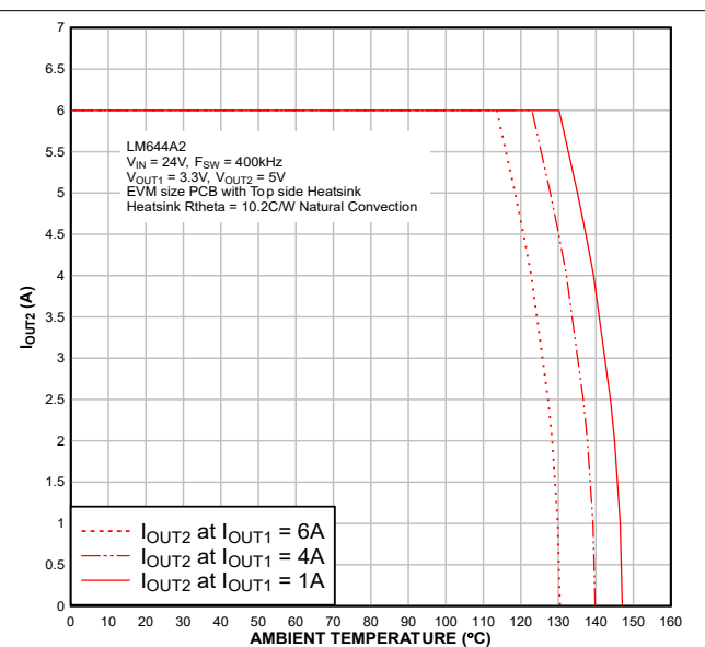
Figure 8-4. Typical Output Current vs Ambient Temperature, V_{IN} = 24V F_{SW} = 400kHz , Dual Output
