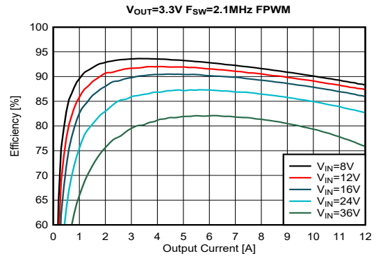
Figure 8-18. Efficiency
