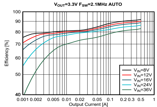
Figure 8-16. Efficiency
