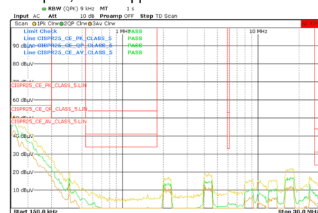
CISPR 25 Conducted, V_{\text{OUT}} = 3.3\text{V} , 2.1MHz, 12A
