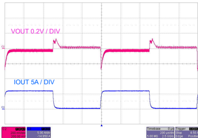
Figure 8-51. Load Transient
