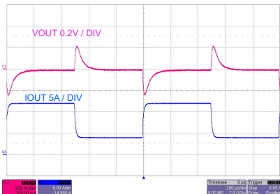
Figure 8-53. Load Transient
