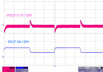
Figure 8-52. Load Transient
