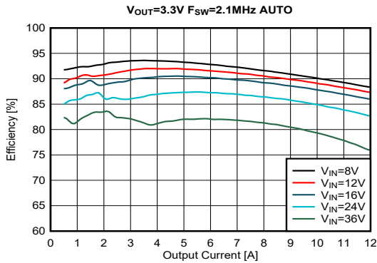
Figure 8-17. Efficiency
