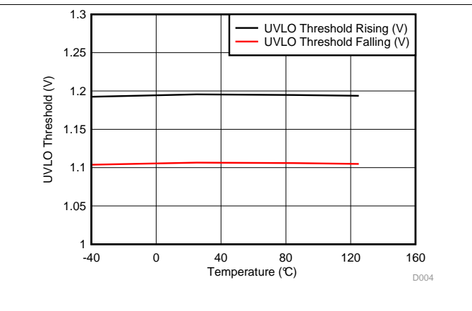
Figure 4. UVLO Thresholds ( V_{UVLOR} , V_{UVLOF} ) vs Temperature
