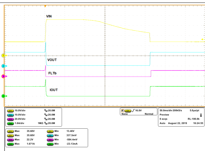
Figure 43. Protection from ISO 16750-2 Pulse 5b [12 V Battery, Transient Voltage = 35 V, R_{LOAD} = 14 \Omega ]
