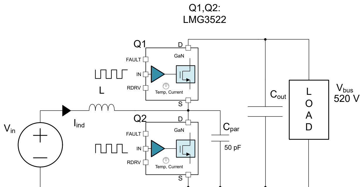
Figure 7-8. Circuit Used for SOA Curve
