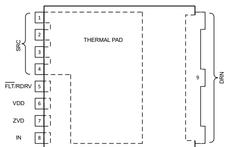
Figure 4-3. LMG3656R025, TOLL Package (Top View)
