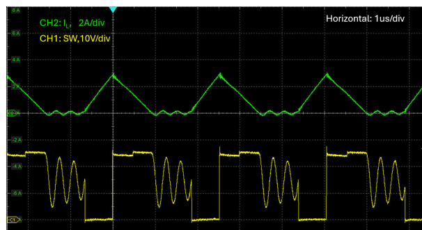
Figure 7-11. V_{in} = 14.4V , V_{out} = 24V , DEM, I_{load} = 0.5A
