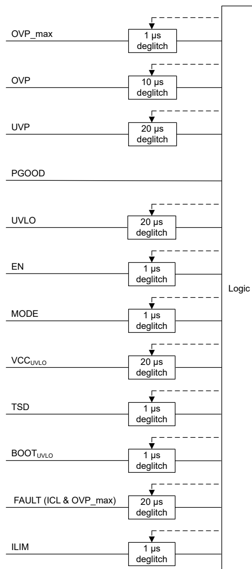
Figure 6-25. Signal Deglitching
