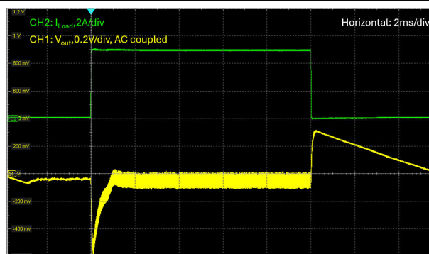
Figure 7-14. Load Transient, V_{in} = 14V , V_{out} = 24V , DEM, I_{load} = 0A to 5A at 1A/\mu s
