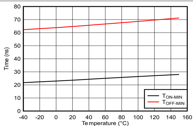
Figure 5-14. Minimum Controllable on Time vs Temperature
