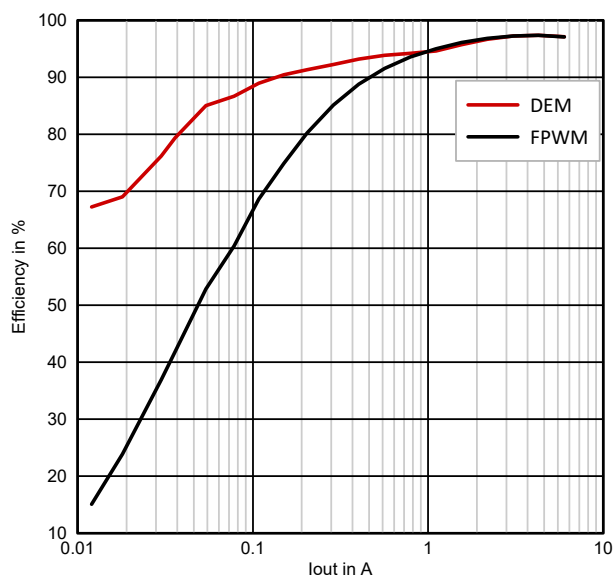
Figure 7-9. Efficiency vs Output Current, V_{in} = 14.4V , V_{out} = 45V
