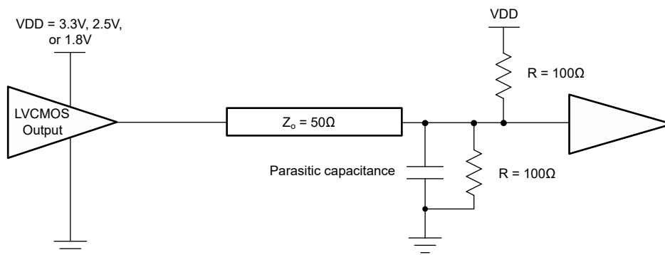
Figure 7-2. Application Load With 50-Ω Termination
