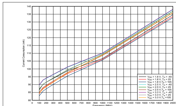
Figure 6-1. LMK1D2104 Current Consumption vs. Frequency
