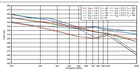
Figure 6-2. LMK1D2104 VOD vs. Frequency
