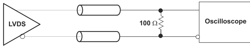
Figure 7-1. LVDS Output DC Configuration During Device Test
