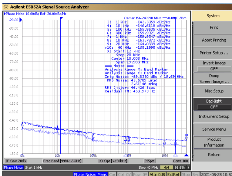
Figure 9-4. LMK1D2104 Output Phase Noise, 156.25MHz, 46.4fs RMS (12kHz to 20MHz)
